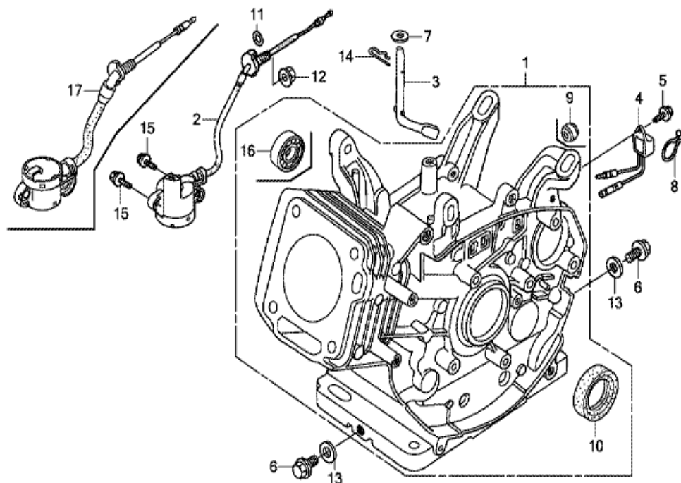
CYLINDER BARREL
